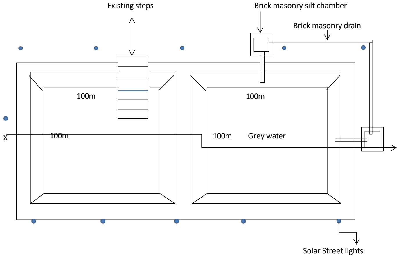
PLAN OF THE POND (Scale-NTS)
