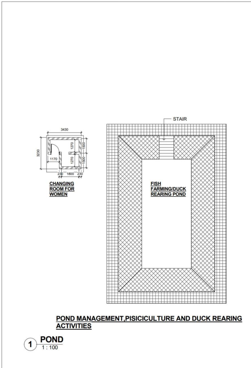
Fig 3:-Diagram for Pond Management
